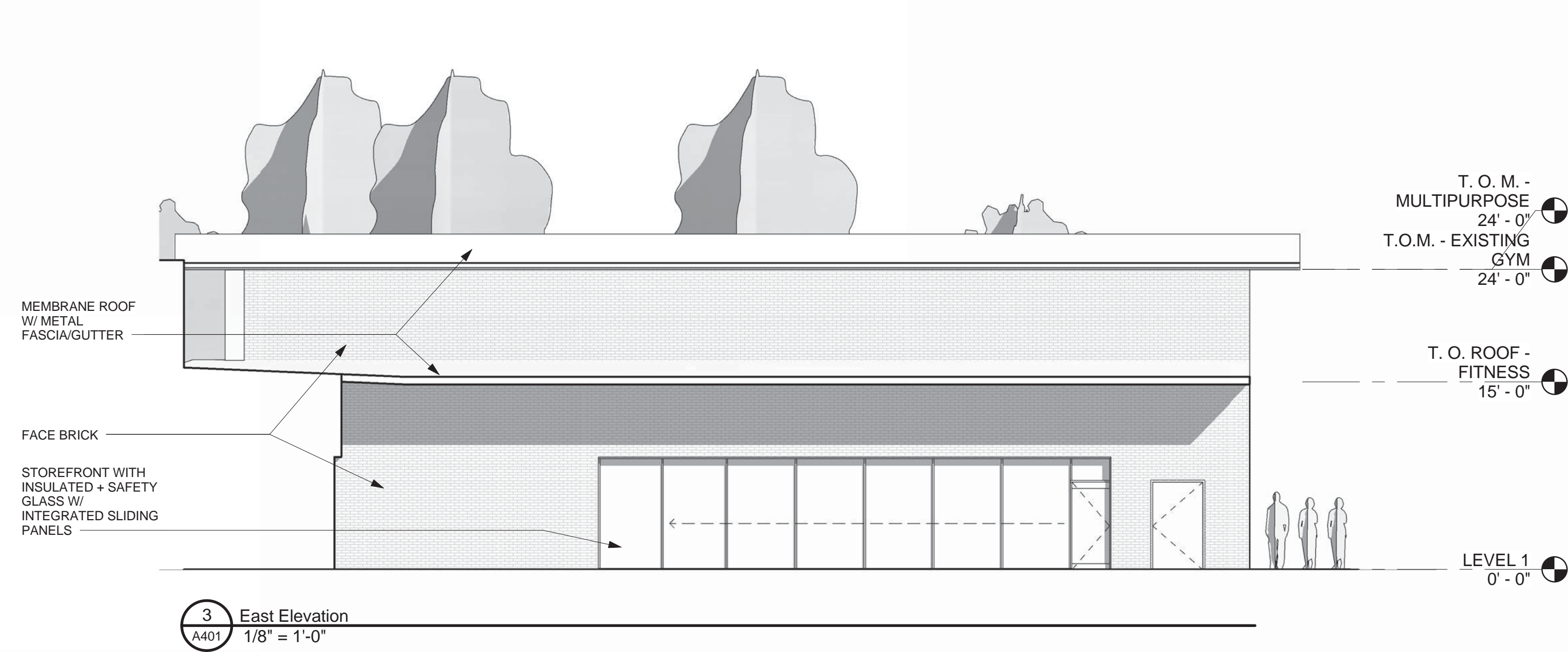
2 North Elevation A401 1/8" = 1'-0"
