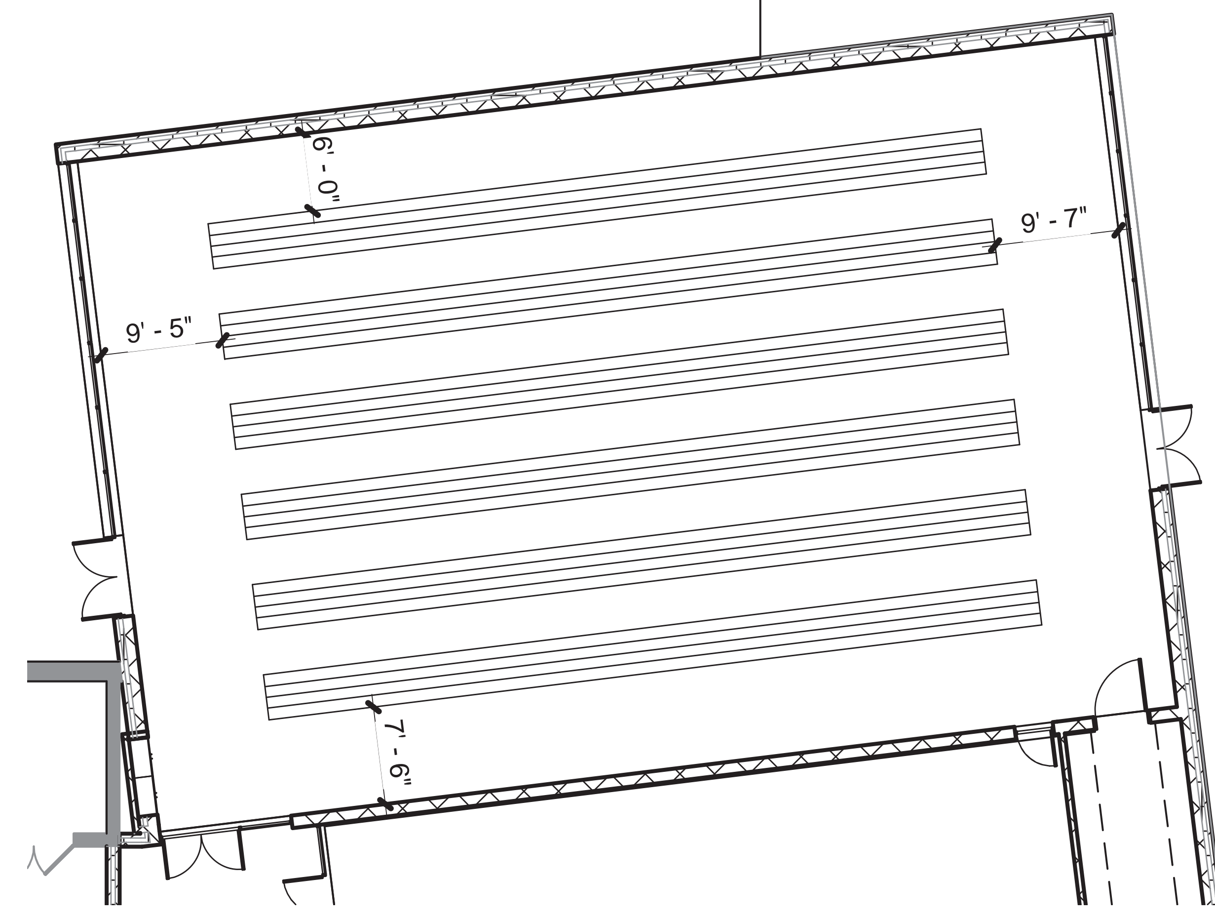
④ MP ROOM: (6) 20 YD SPRINT LANES
