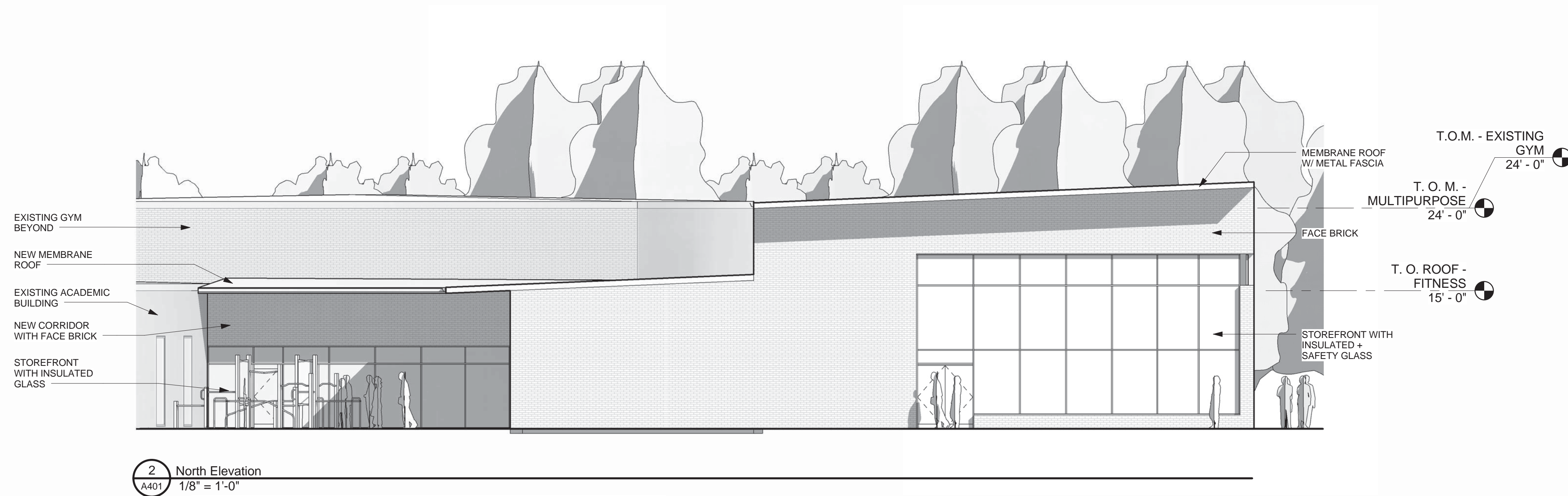
1 West Elevation A401 1/8" = 1'-0"
