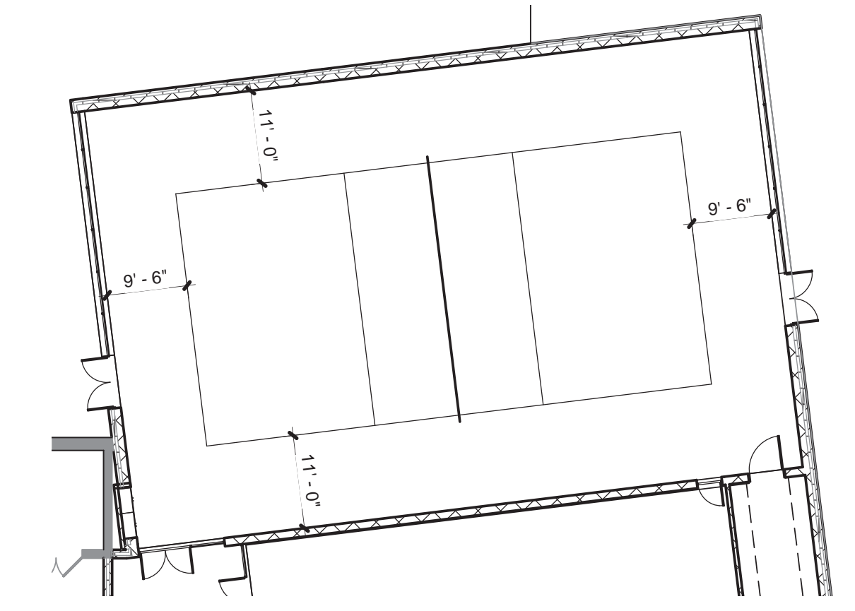
3 MP ROOM: (1) VOLLEYBALL COURT 1/16" = 1'-0"
