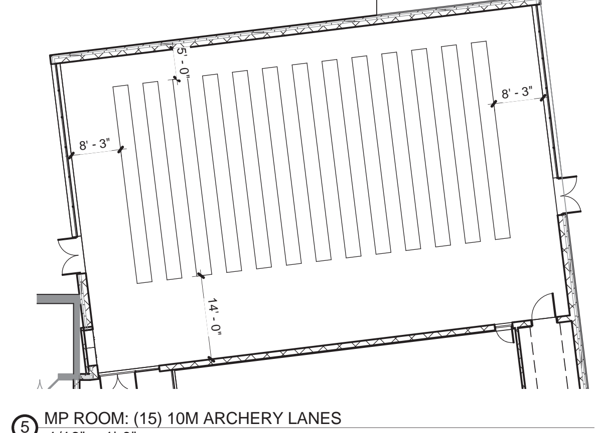
5 MP ROOM: (15) 10M ARCHERY LANES 1/16" = 1'-0"
