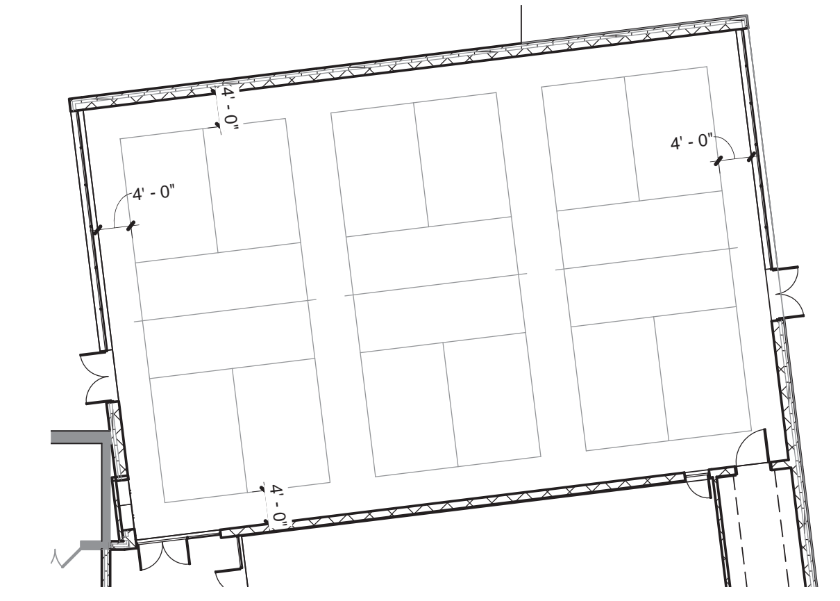
2 MP ROOM: (3) PICKLE BALL COURTS 1/16" = 1'-0"
